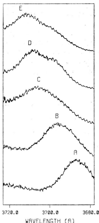
Fig. 1. Spectra of Anthracene-Argon Complexes at A 1.5, B 2.0, C 2.5, D 3.0 and E 3.5 atm of Ar carrier gas. Excitation bandwidth is 0.3 cm -1 .
